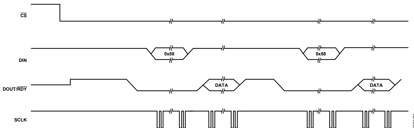
Figure 26. Continuous Conversion
