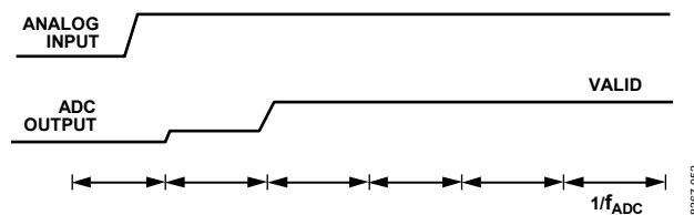
Figure 56. Step Change on Analog Input, \text{Sinc}^4 Filter
